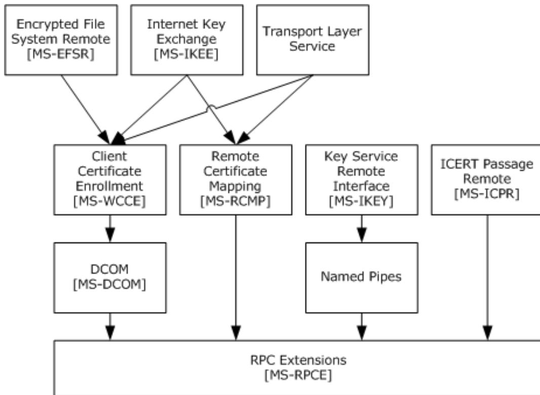
Figure 23: Protocol interdependencies
