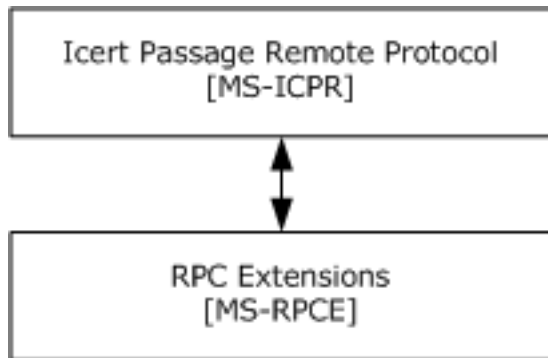
Figure 21: ICertPassage
