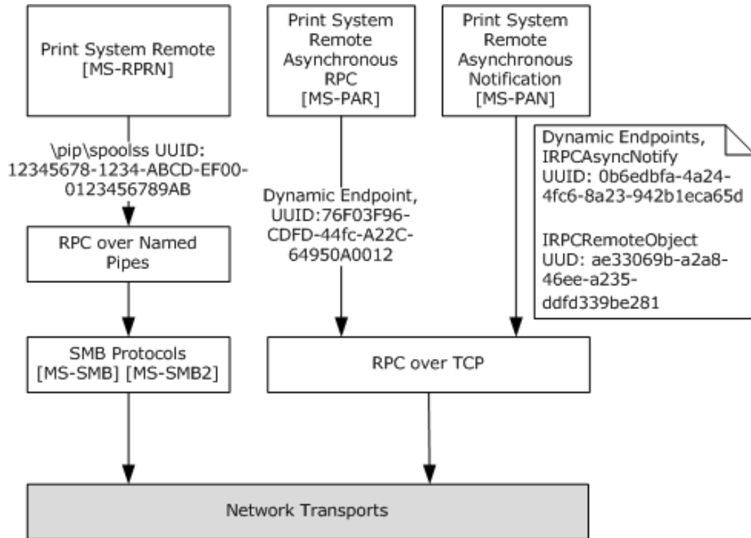
Figure 7: Combined protocol stack
