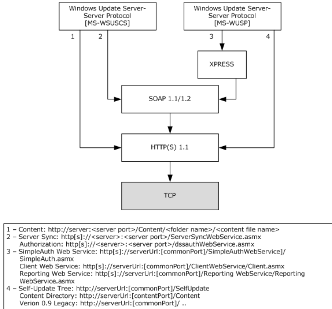
Figure 27: Windows Update services
