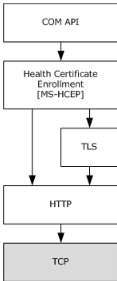
Figure 38: Client-side protocol stack
