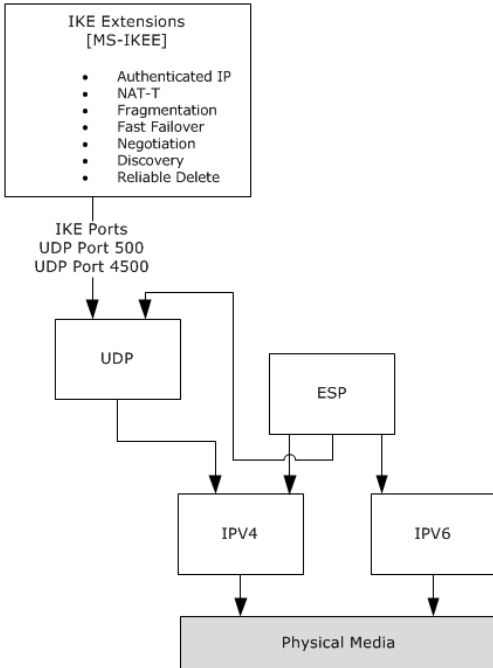
Figure 50: IKE Protocol Extensions
