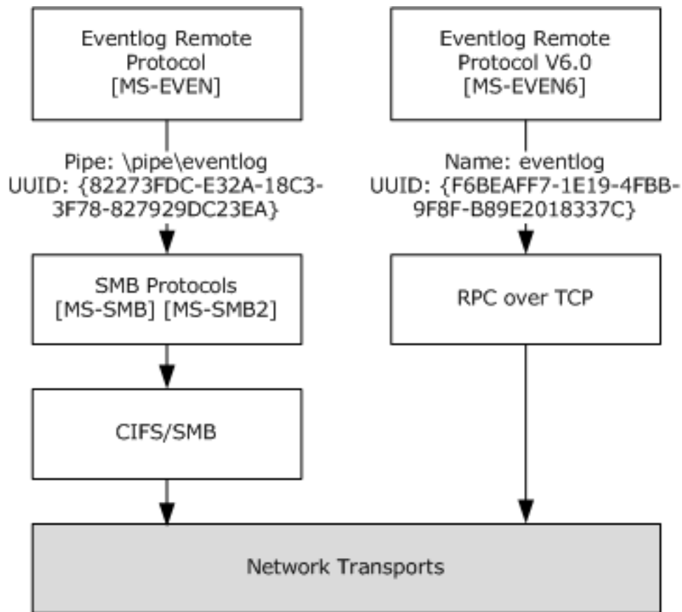
Figure 32: Eventlog Remote Protocol
