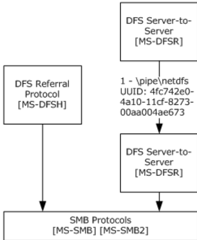
Figure 5: Protocol stack
