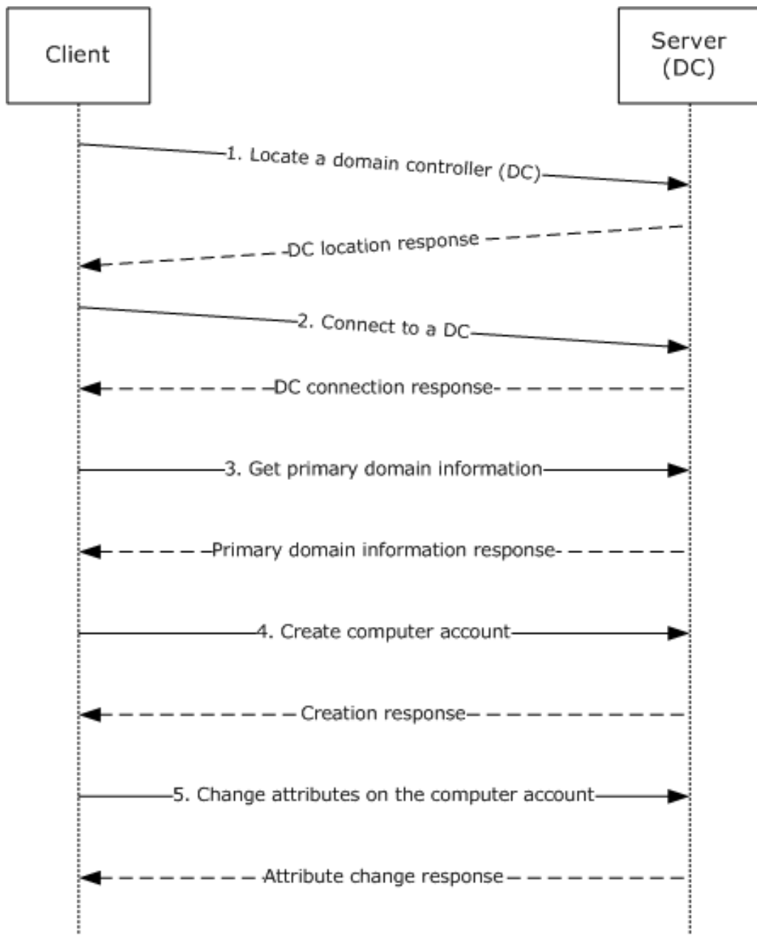
Figure 52: Message sequencing
