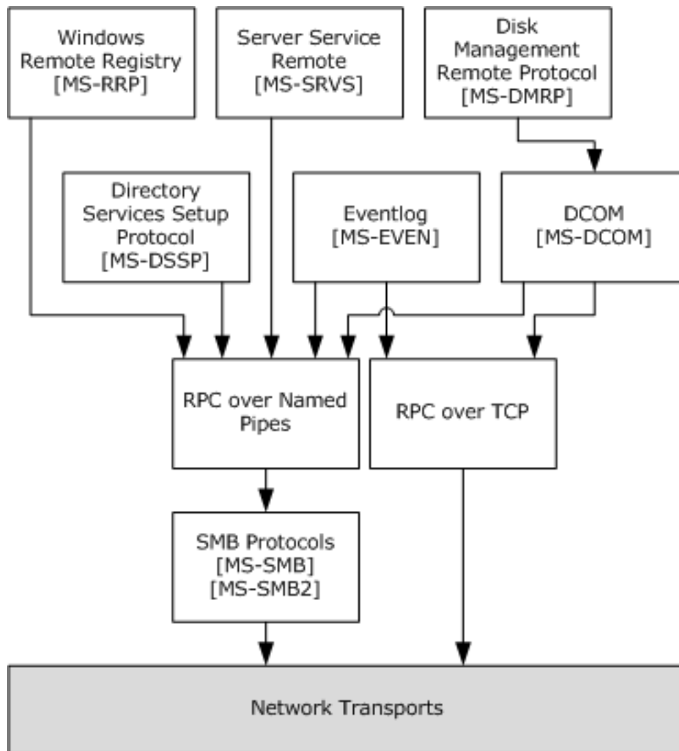
Figure 25: Protocol scenarios
