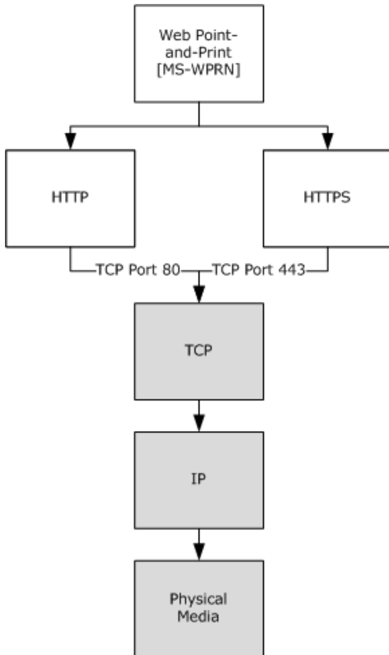
Figure 8: Protocol layering
