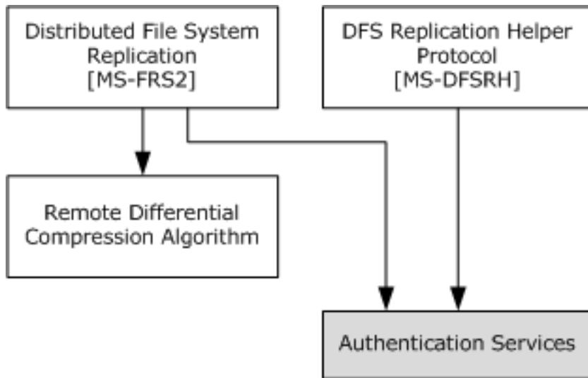
Figure 10: Logical dependencies
