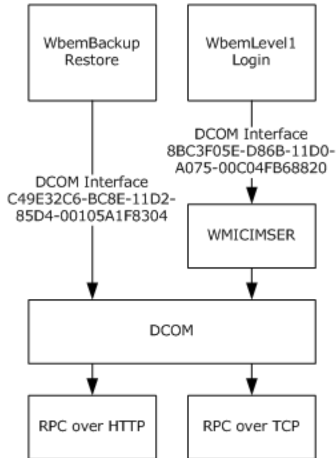
Figure 51: Protocol stack
