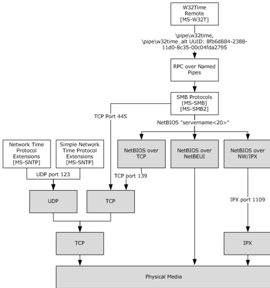
Figure 33: Layered protocols
