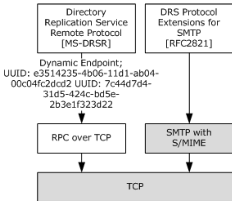
Figure 28: Protocol stack
