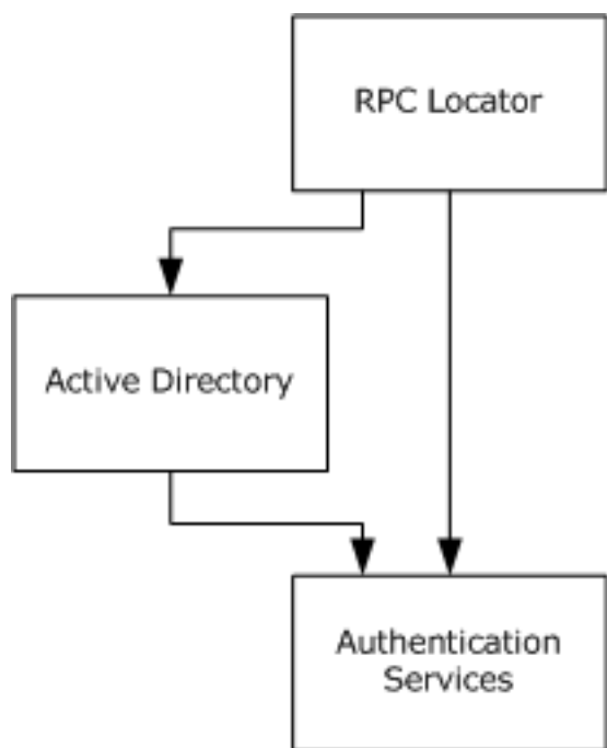
Figure 37: RPC dependencies
