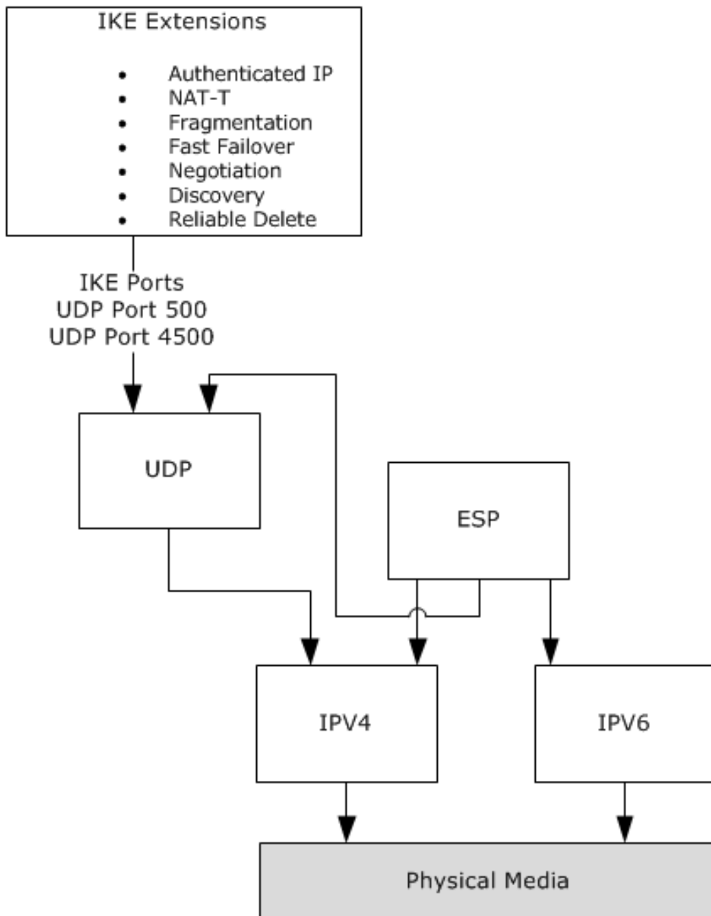
Figure 16: Scenario extensions
