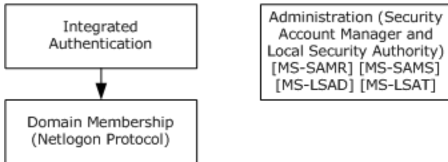
Figure 17: Basic authentication
