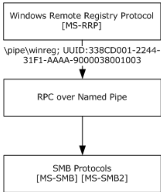
Figure 31: Protocol stack
