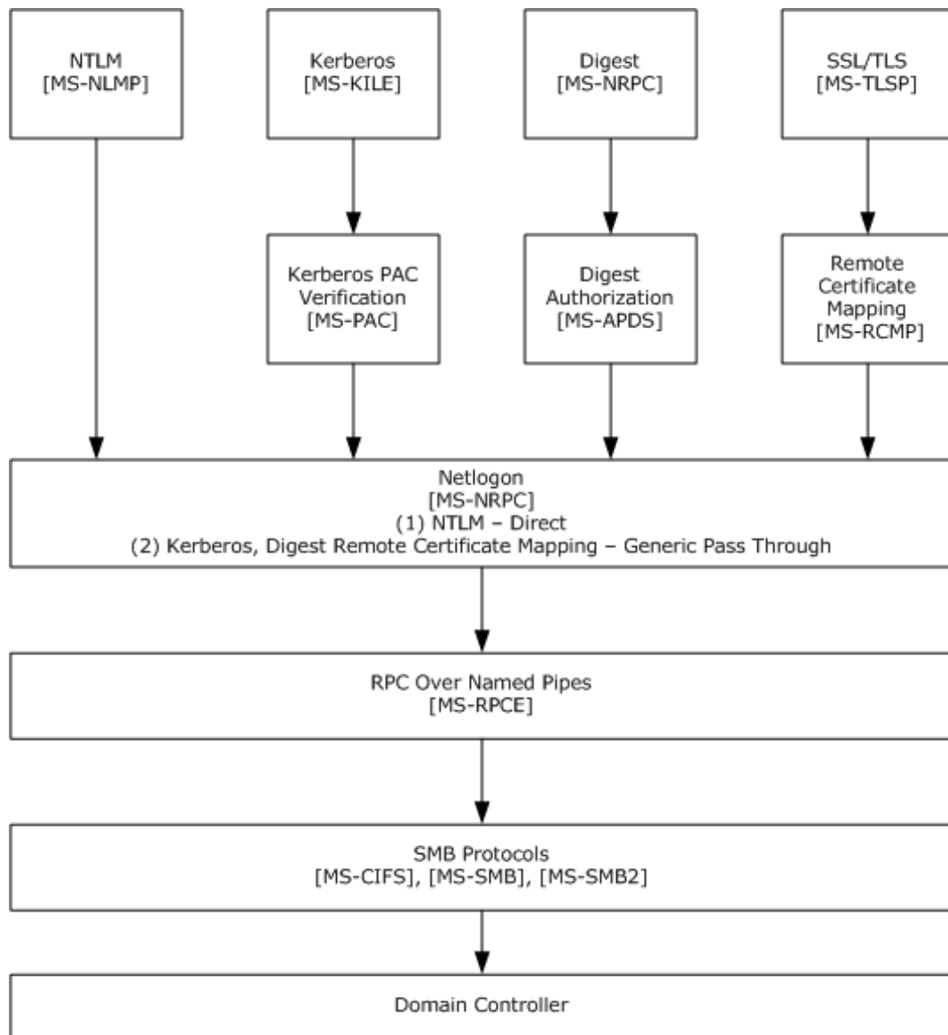
Figure 18: Domain-based authentication
