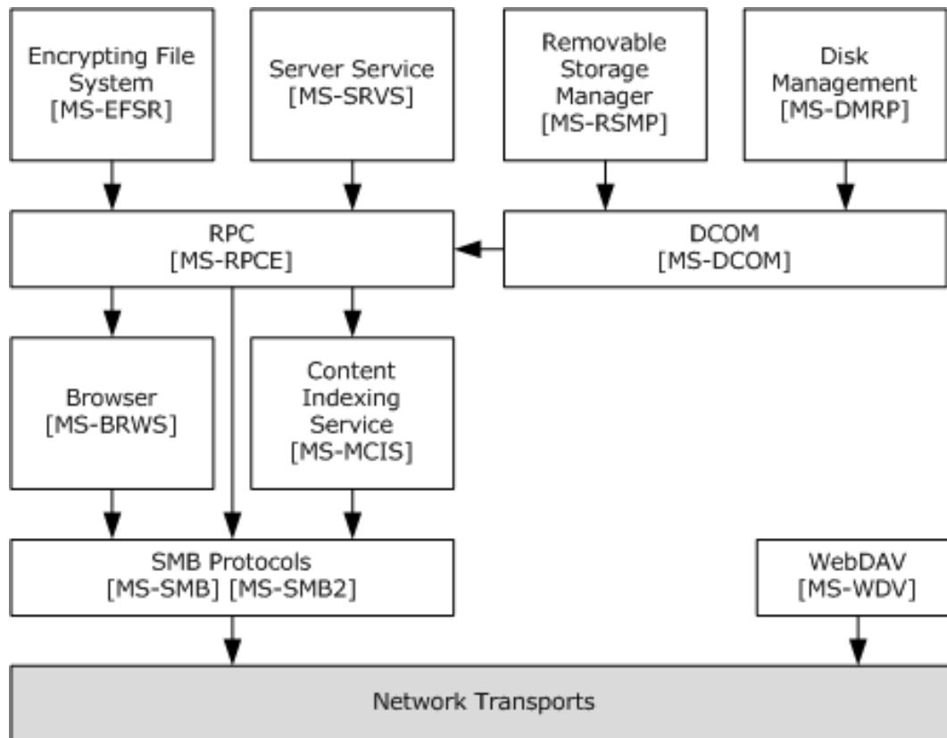
Figure 1: Remote file access protocols
