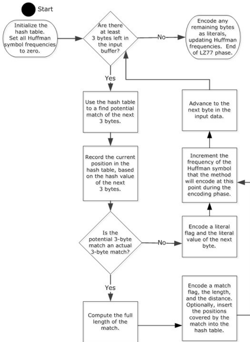
Figure 1: LZ77 phase
