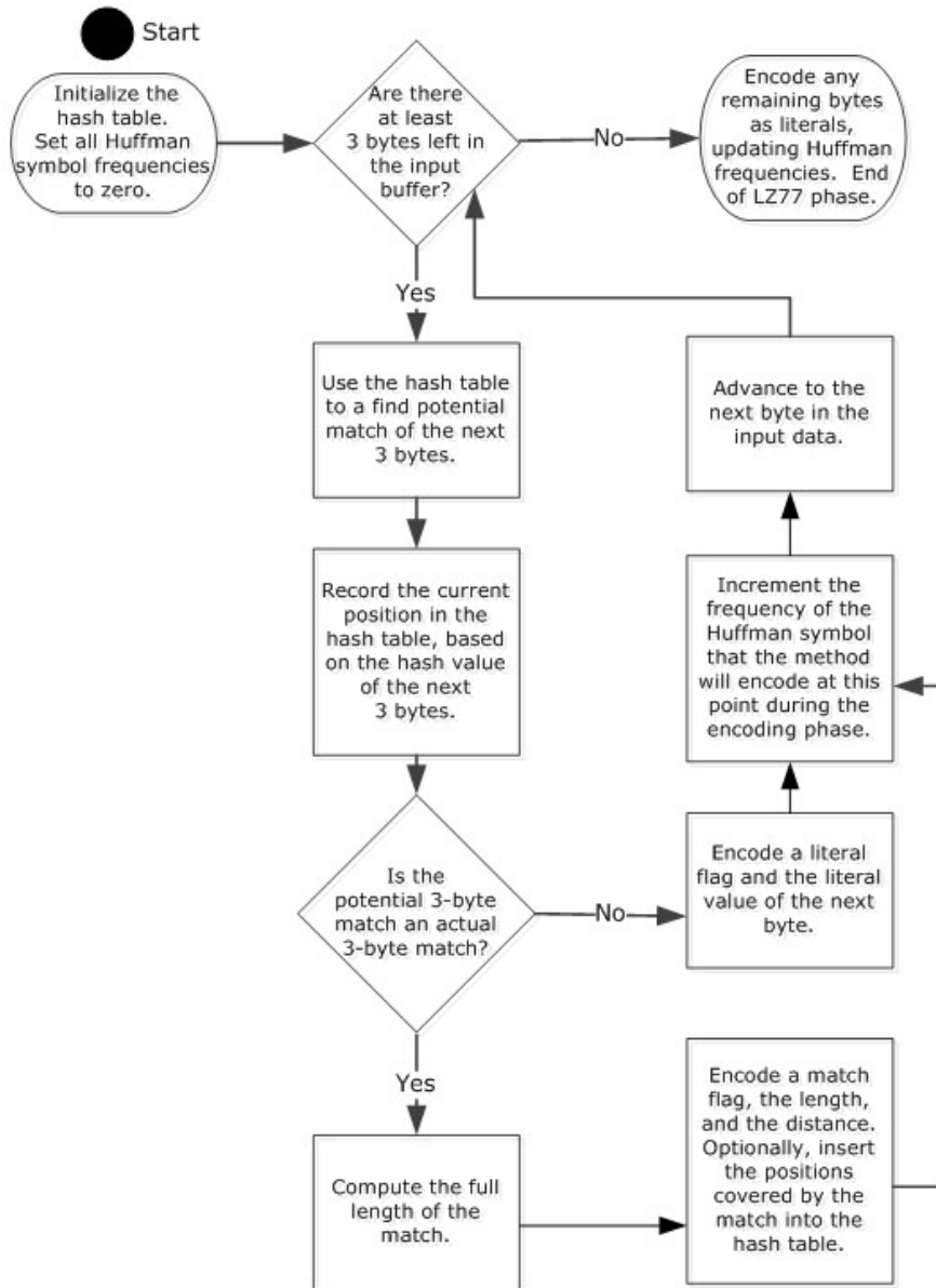
Figure 1: LZ77 phase
