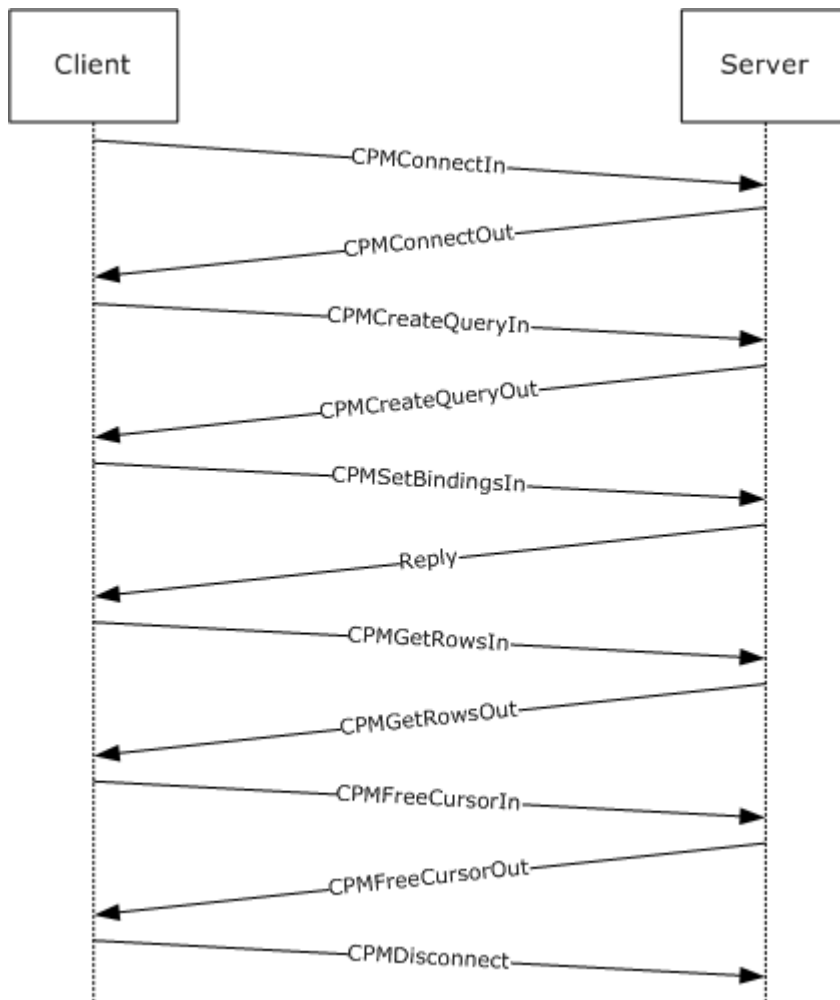
Figure 5: Windows Search Protocol session life cycle
