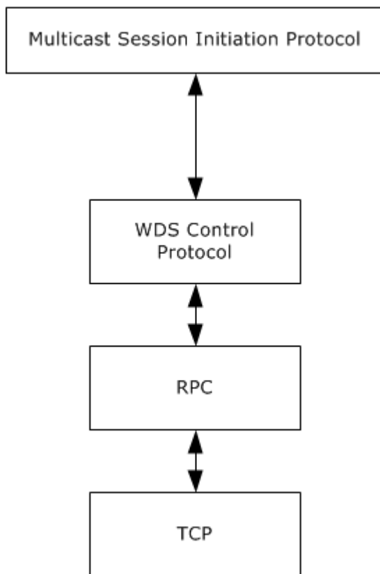
Figure 1: Protocol relationships
