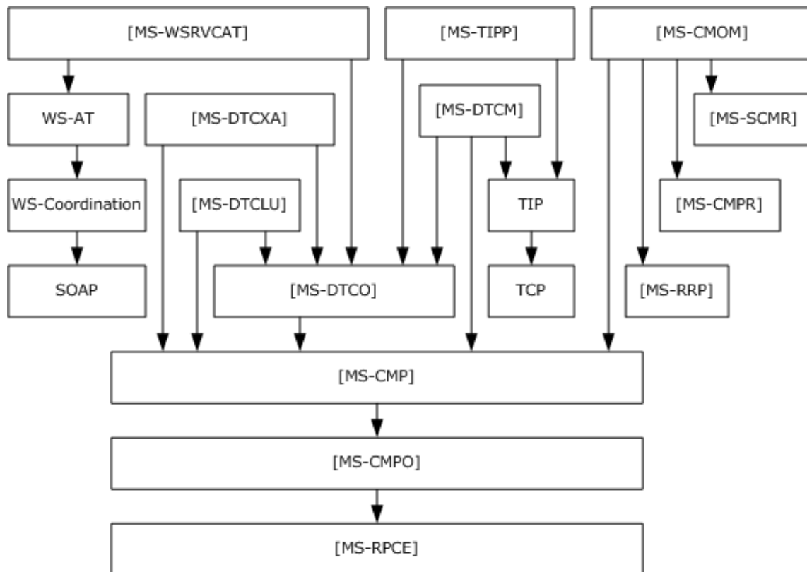
Figure 5: Transaction processing services protocol dependencies
