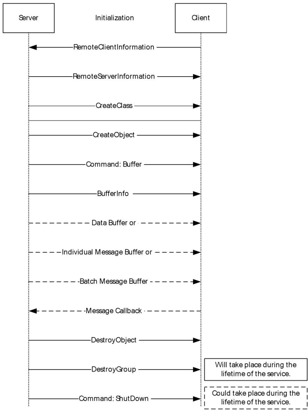
Figure 3: Message sequence
