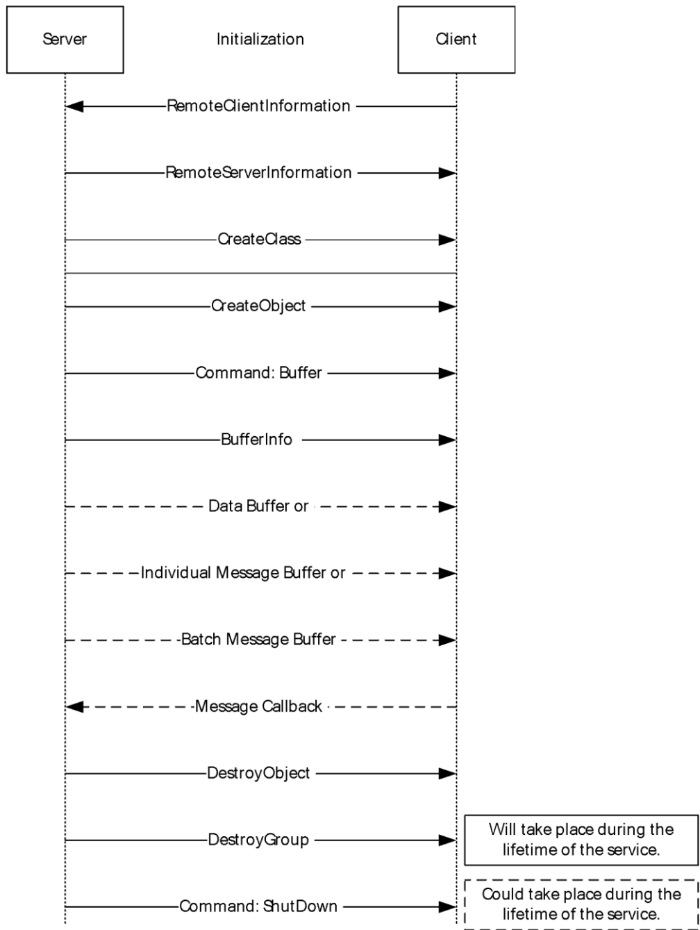
Figure 3: Message sequence
