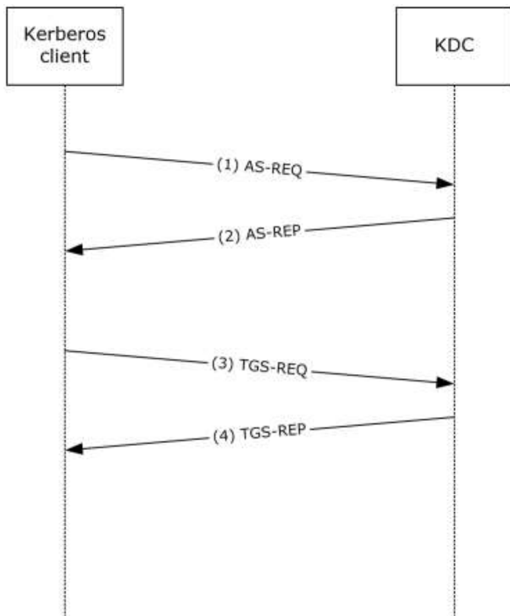
Figure 1: Interactive logon
