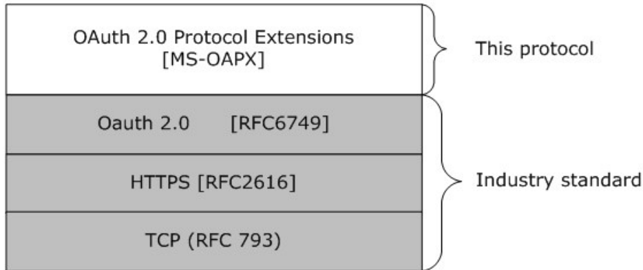
Figure 1: Protocol dependency
