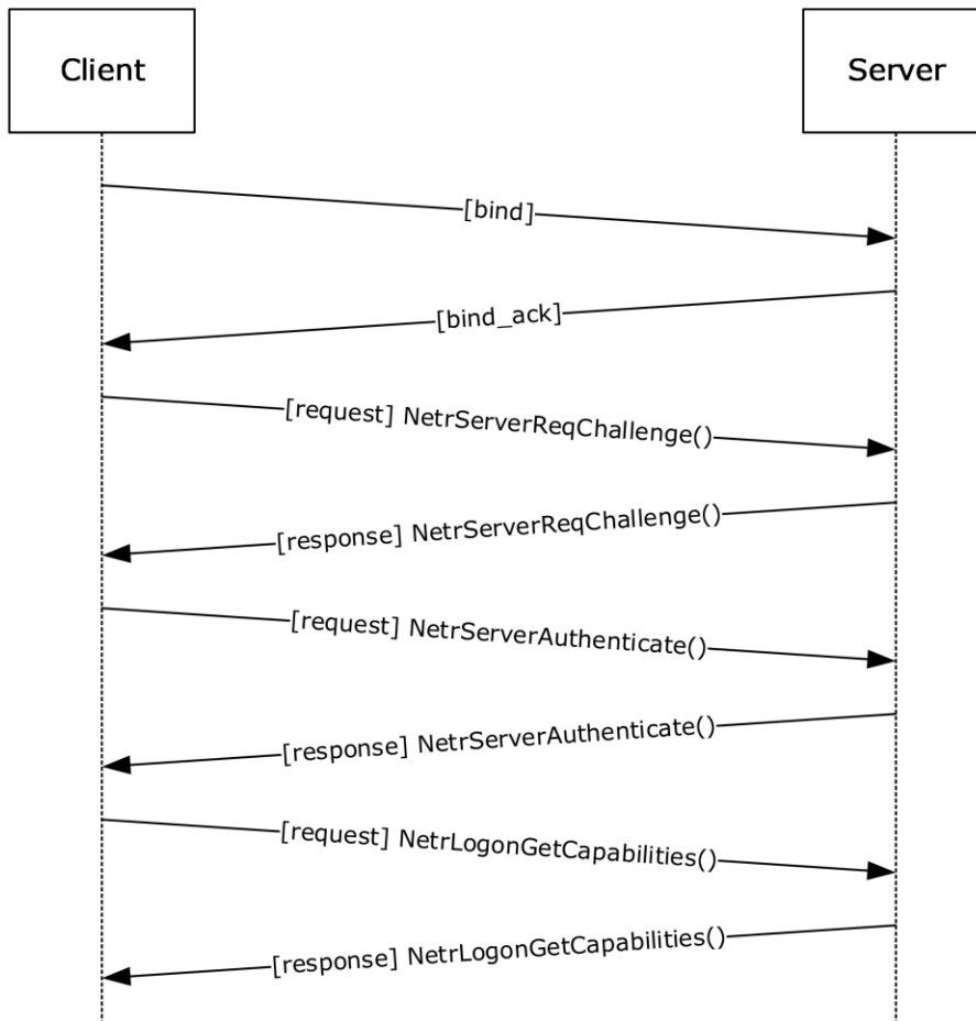
Figure 76: Session-key negotiation
