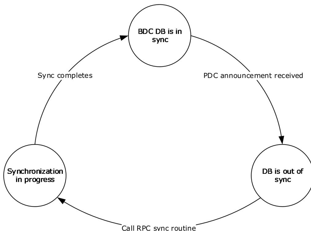
Figure 98: BDC States
