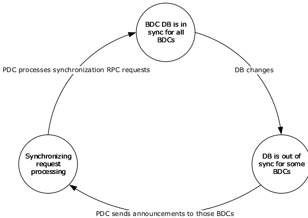
Figure 87: PDC States
