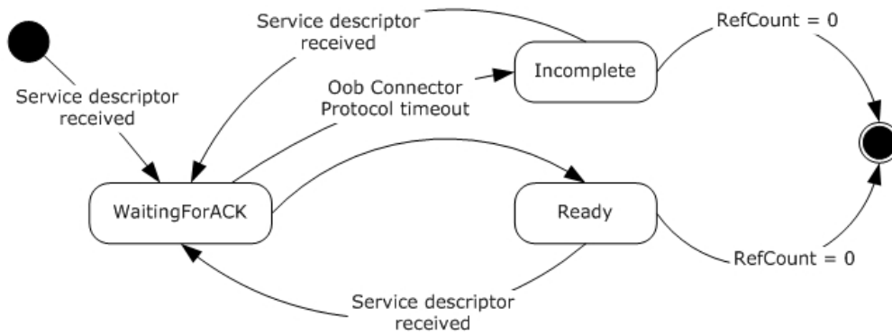
Figure 4: OOB Connector state transitions: Connector role
