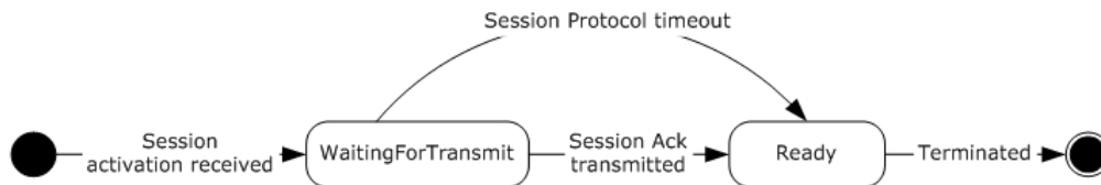
Figure 8: Session state transitions: Server role
