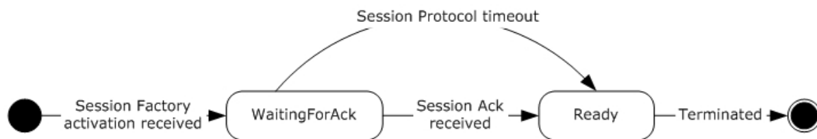
Figure 7: Session state transitions: Client role
