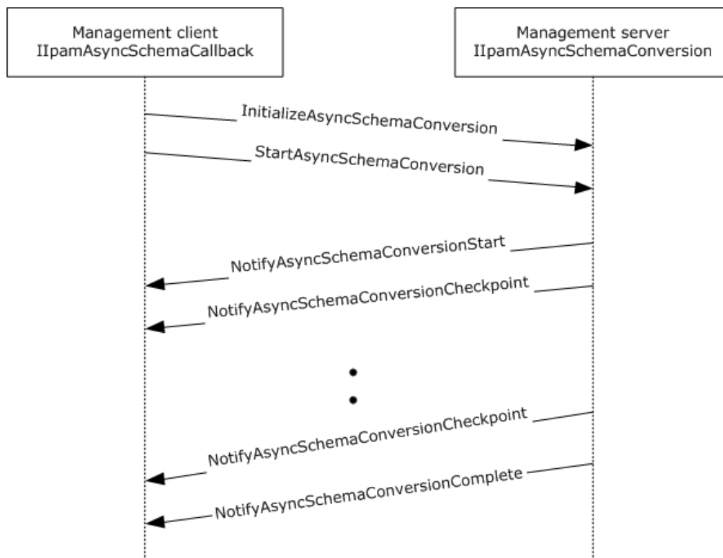
Figure 9: Schema Conversion - Protocol Interaction
