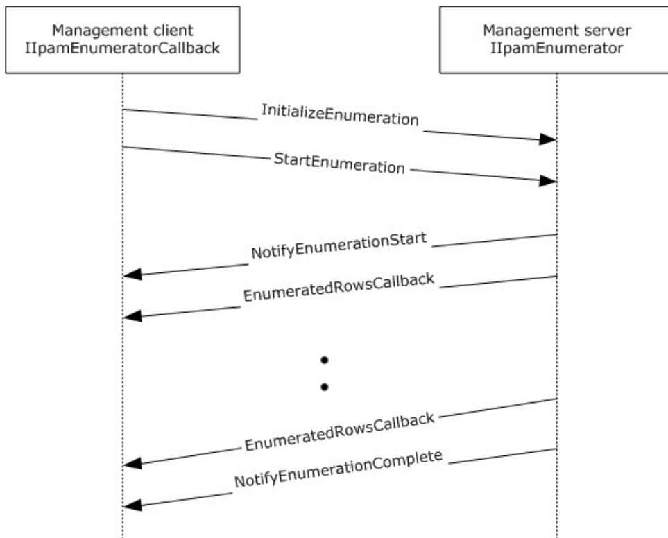
Figure 3: Enumeration Callback Interaction
