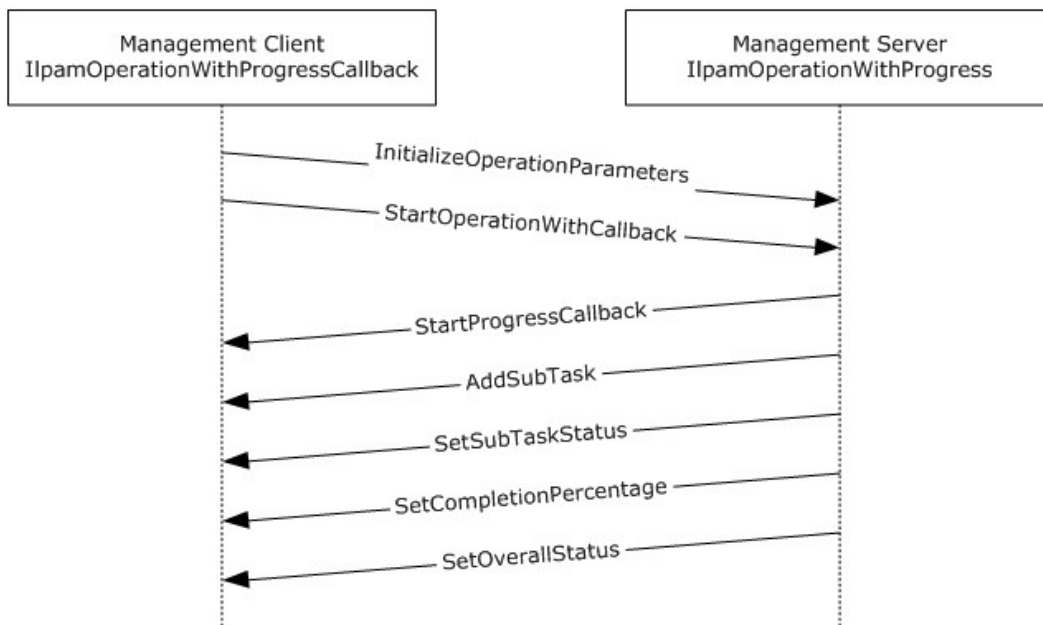
Figure 12: OperationWithProgress interaction
