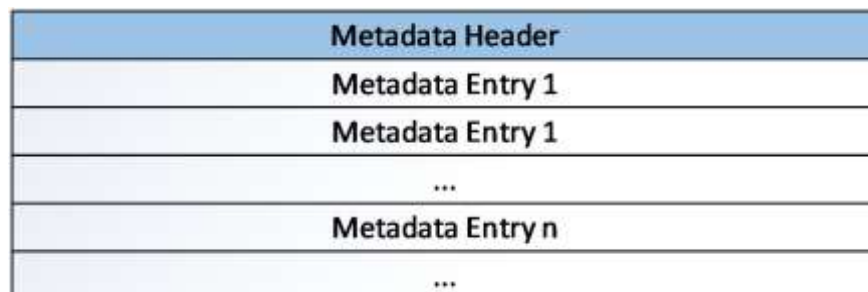
Figure 2: Metadata structure
