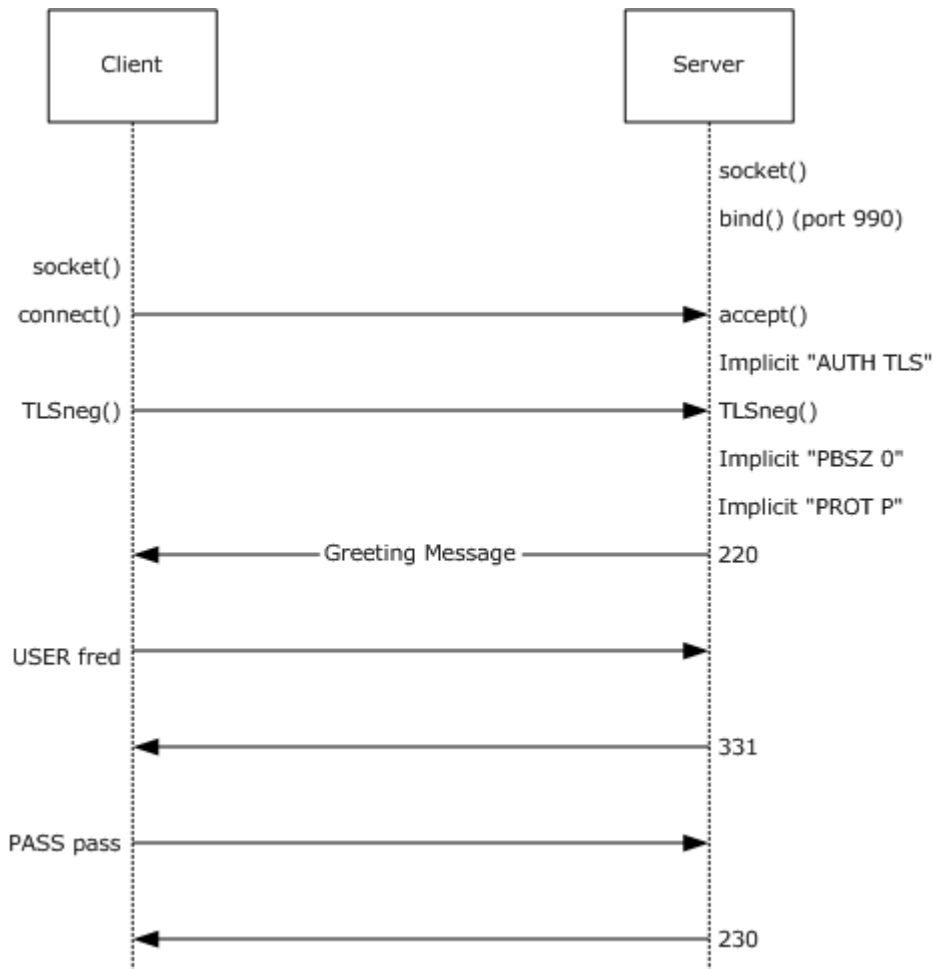
Figure 1: Control connection negotiation with Implicit FTPS
