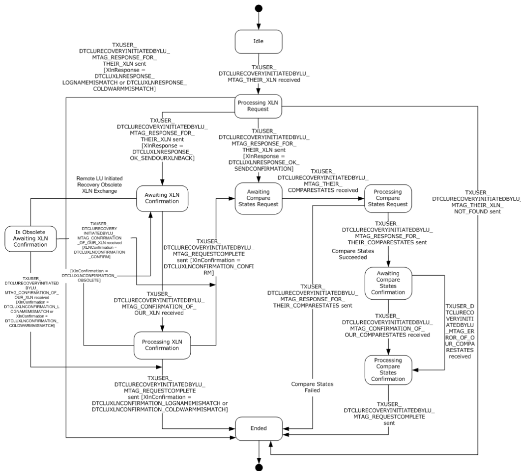
Figure 18: CONNTYPE_TXUSER_DTCLURECOVERYINITIATEDBYLU acceptor states
