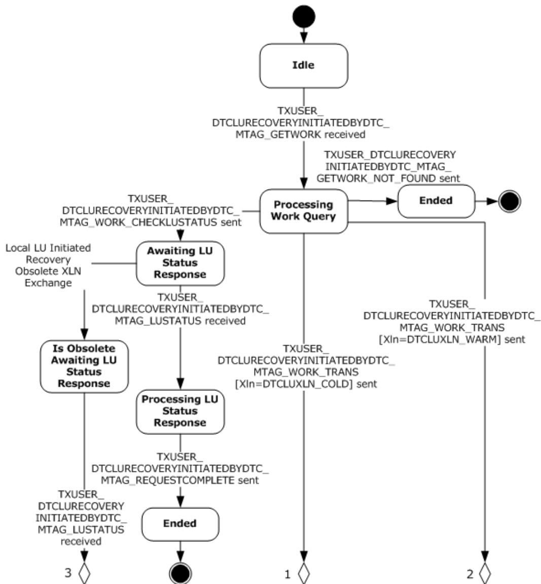
Figure 14: CONNTYPE_TXUSER_DTCLURECOVERYINITIATEDBYDTC, Part 1
