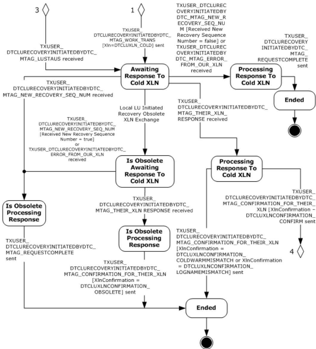
Figure 15: CONNTYPE_TXUSER_DTCLURECOVERYINITIATEDBYDTC, Part 2
