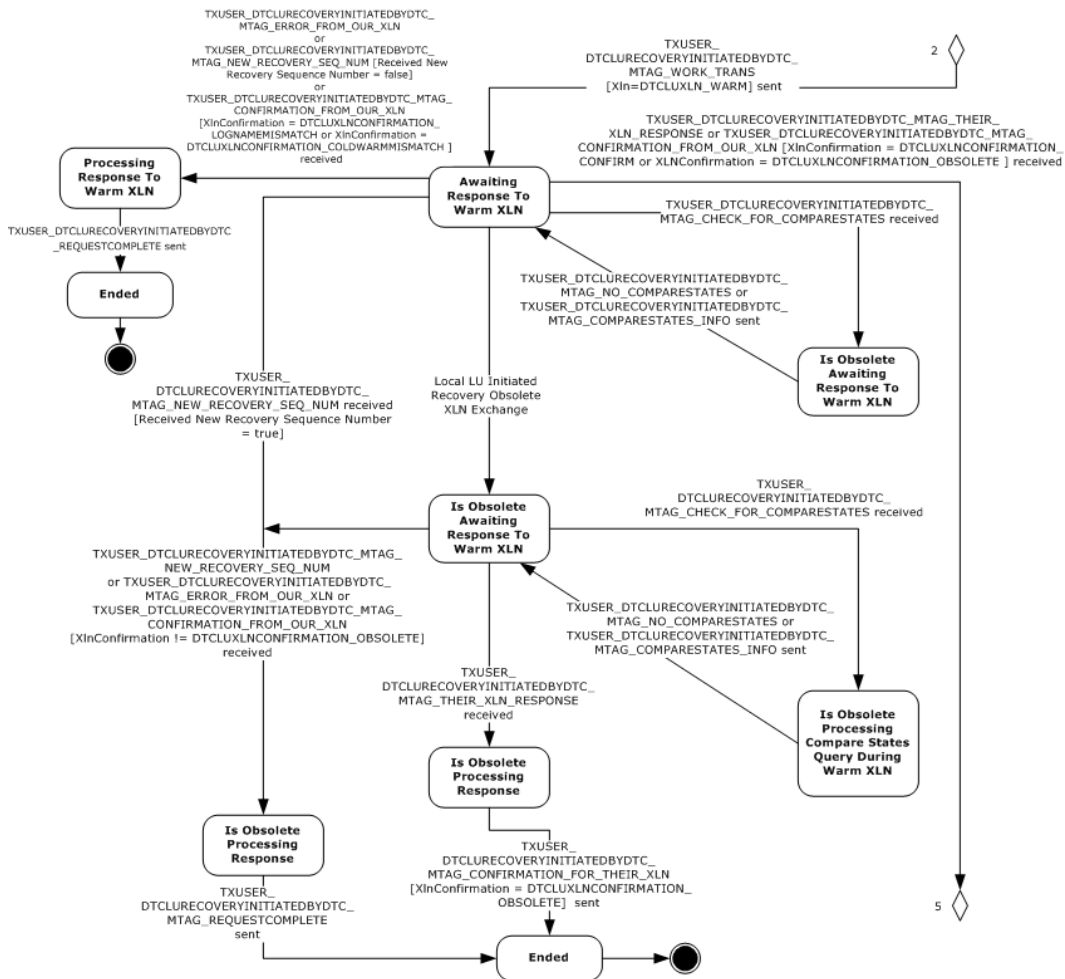
Figure 16: CONNTYPE_TXUSER_DTCLURECOVERYINITIATEDBYDTC, Part 3
