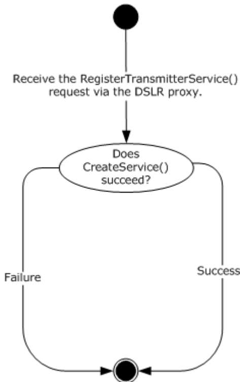
Figure 3: RegisterTransmitterService operation
