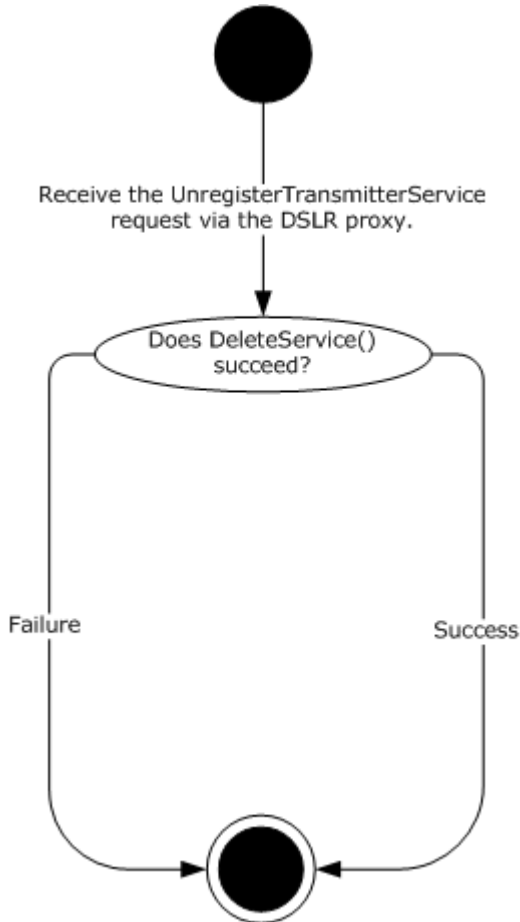
Figure 4: UnregisterTransmitterService operation
