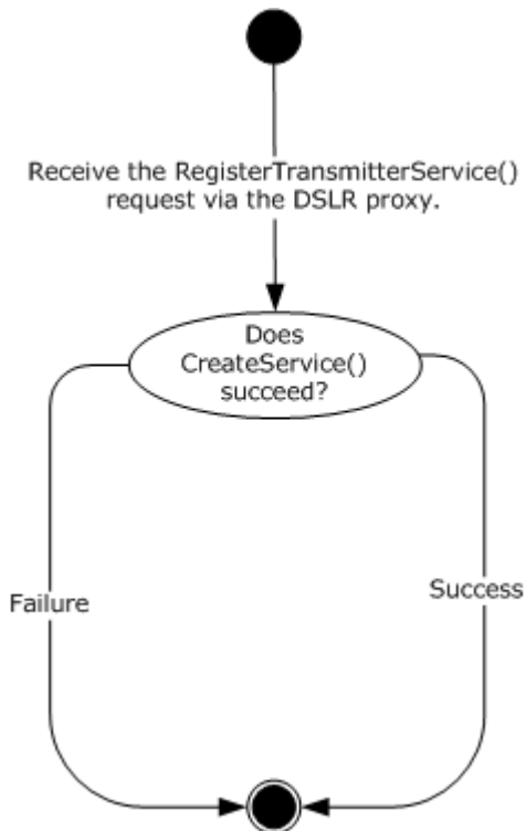
Figure 3: RegisterTransmitterService operation
