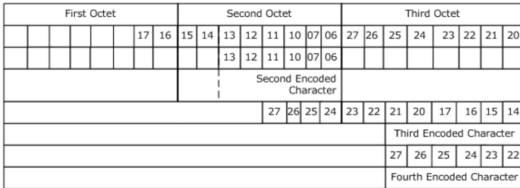
Figure 2: Data encoding of the lowest 6 bits and remaining 4 bits
