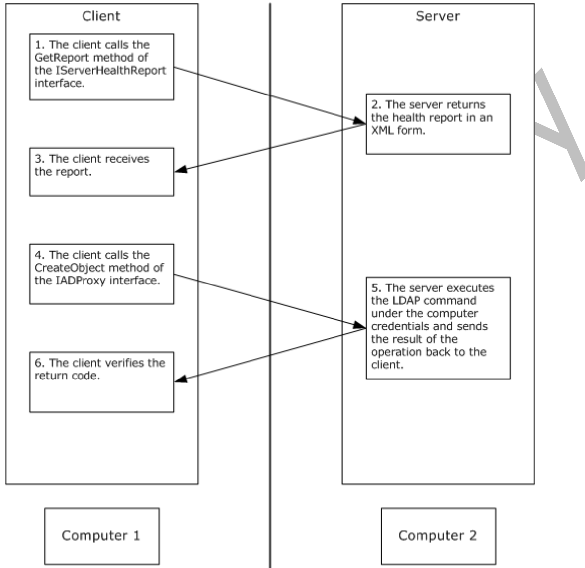
Figure 1: Example of messages between a client and server
