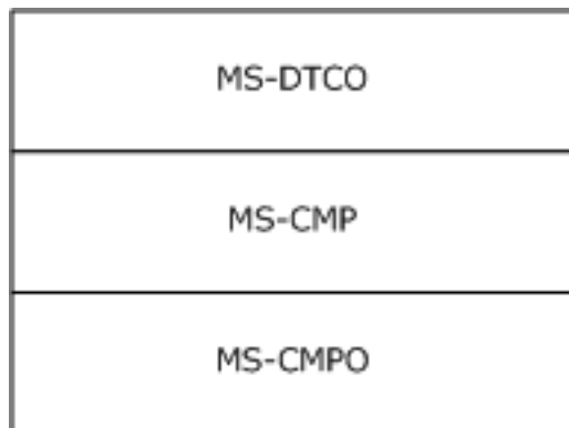
Figure 3: Protocol relationships
