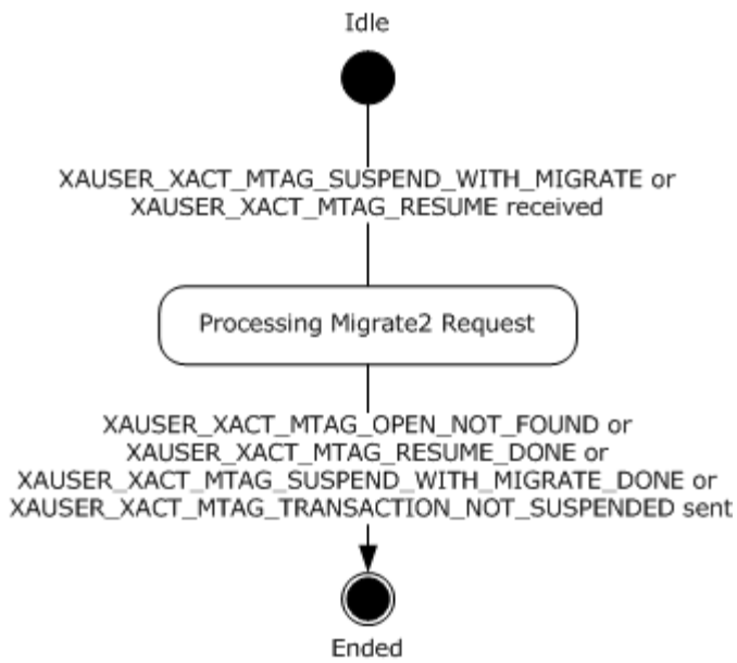
Figure 18: CONNTYPE_XAUSER_XACT_MIGRATE2 acceptor states
