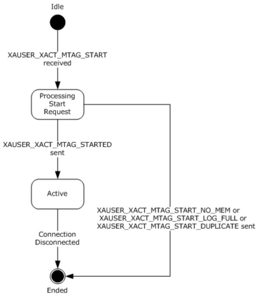
Figure 16: CONNTYPE_XAUSER_XACT_BRANCH_START acceptor states
