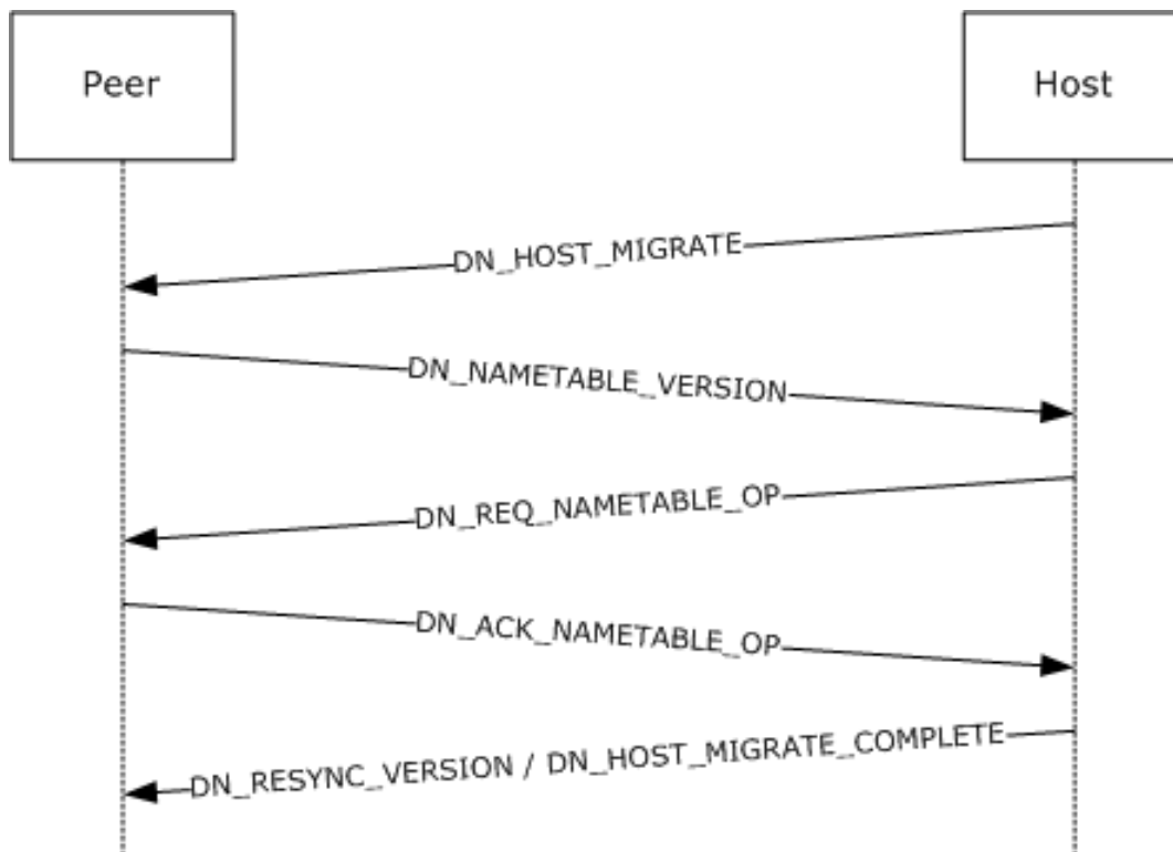
Figure 15: Peer-to-peer host disconnect (possible host migration)
