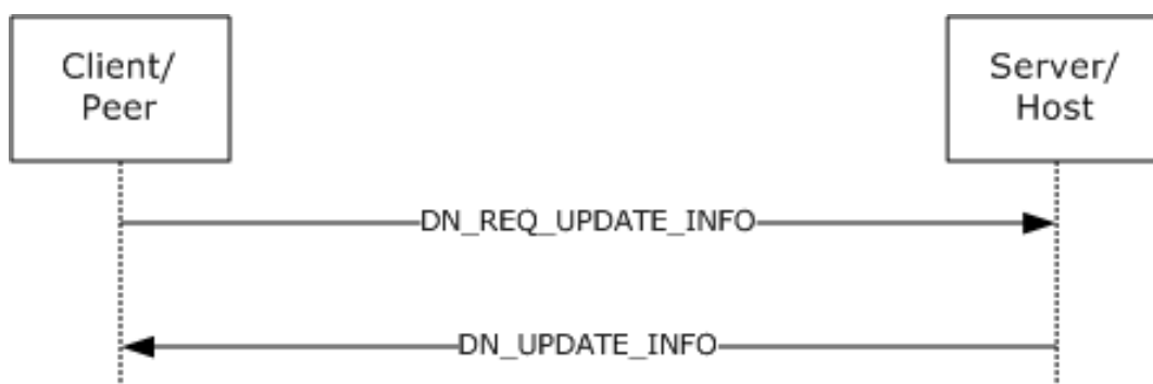
Figure 21: Update Information Sequence Diagram
