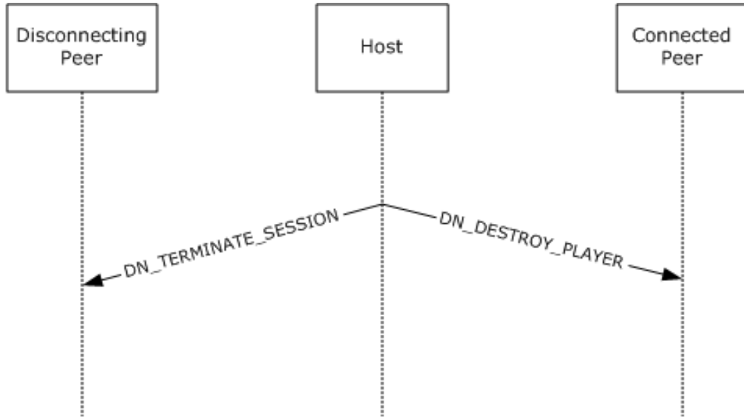
Figure 13: Peer-to-peer host disconnect sequence
